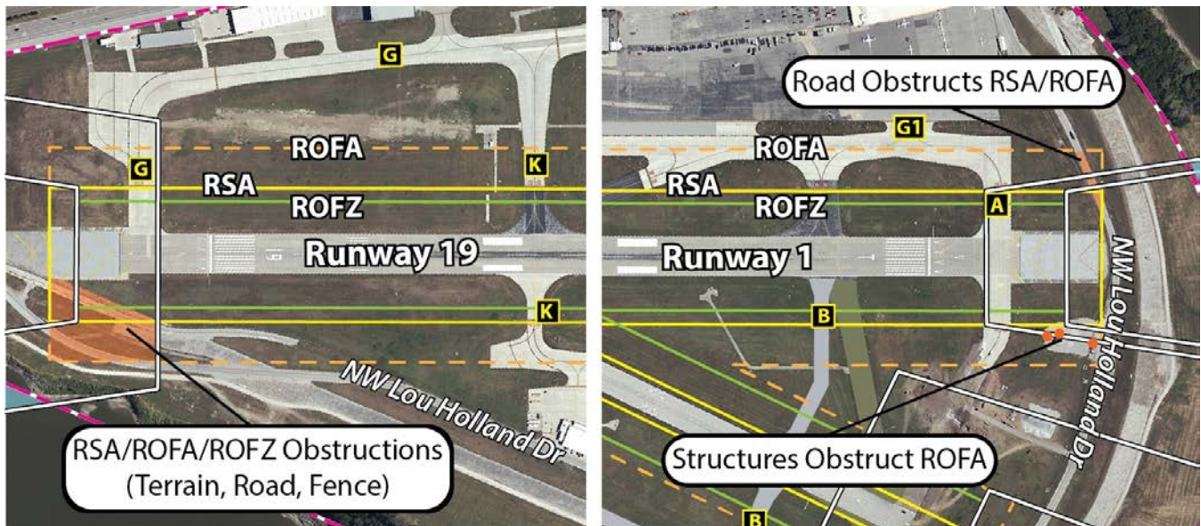
Exhibit 4B – Non-standard Safety Areas (Runway 1-19)
