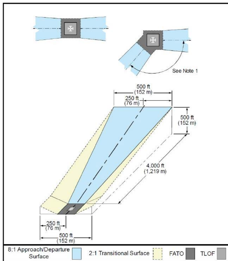
Figure 4-2: Vertiport Design Considerations
