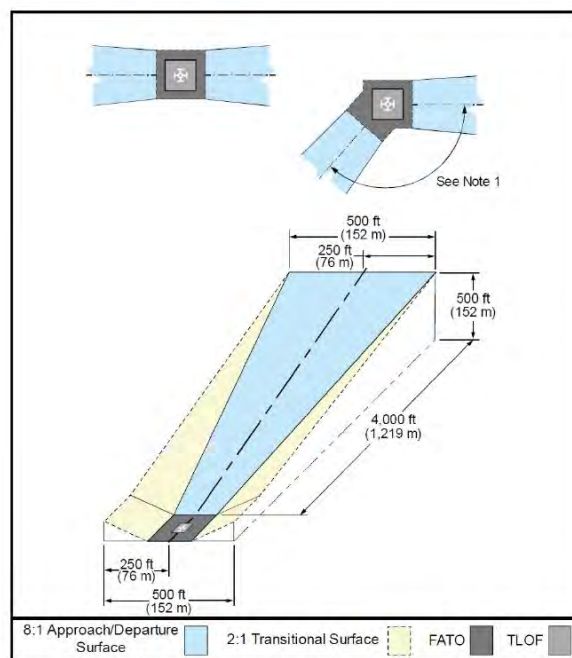
Figure 4-2: Vertiport Design Considerations
